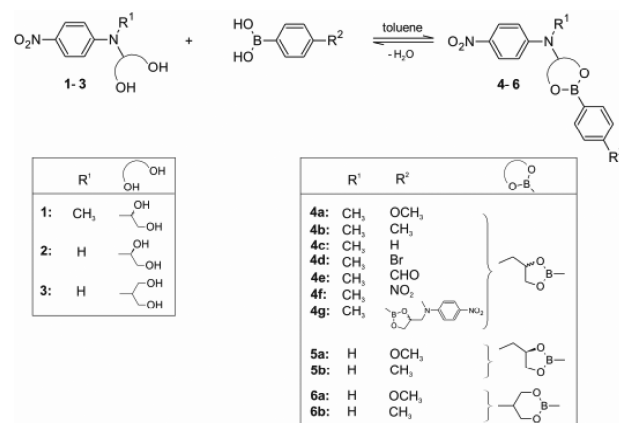
Scheme 2. Synthesis of the Boronic Acid Esters 4–6
