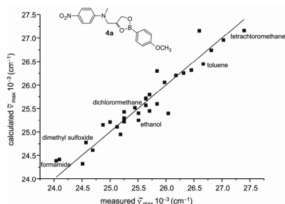
Figure 3. Relationship between calculated and measured \tilde{\nu}_{\max} values for 4a, according to the Kamlet–Taft equation (eq 1).
